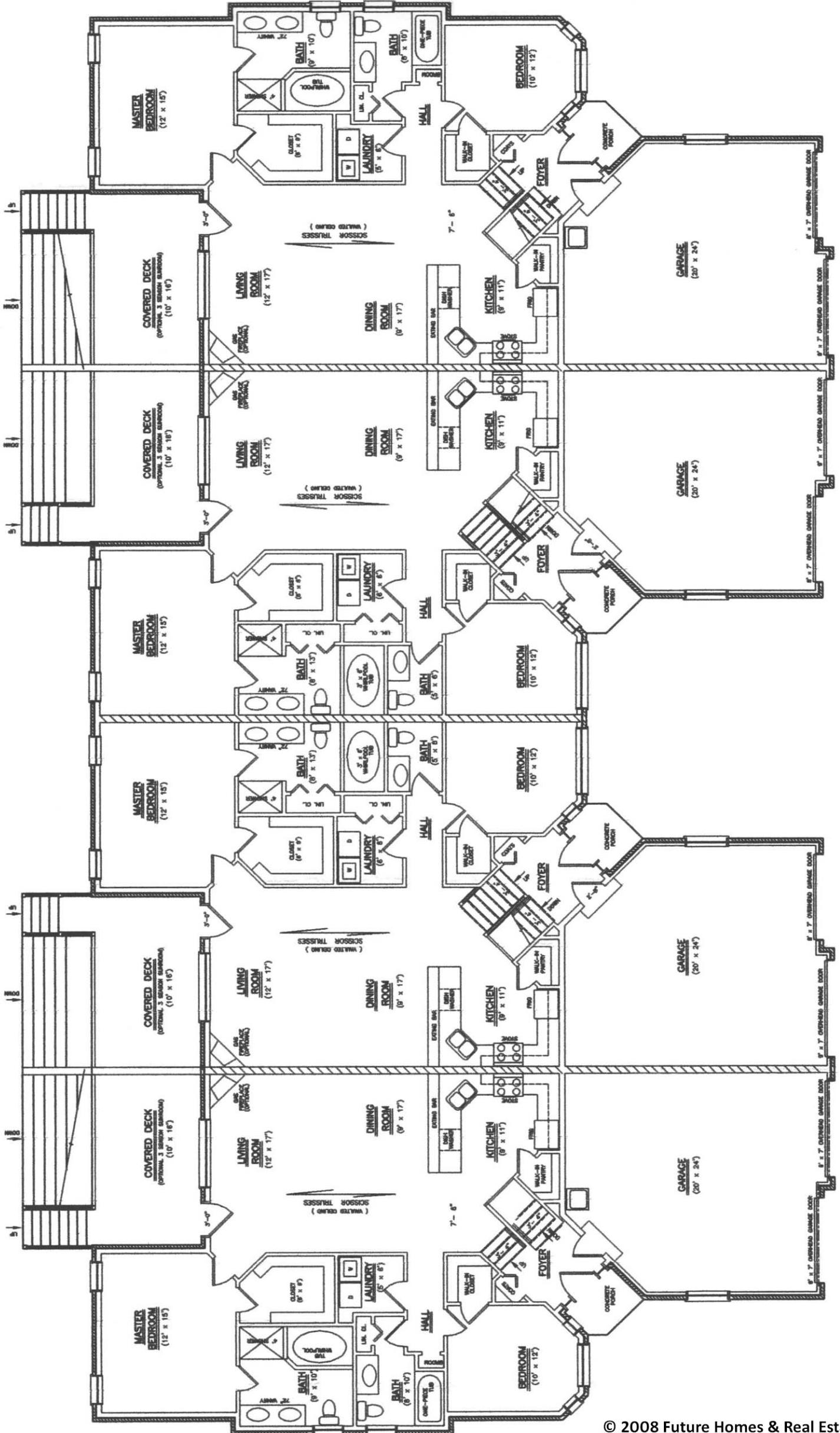
FLOOR PLAN (END UNIT-1330 SQ. FT.+ COVERED DECK) (GAR.-495 SQ. FT.) (PARTIALLY RAISED-RANCH)
